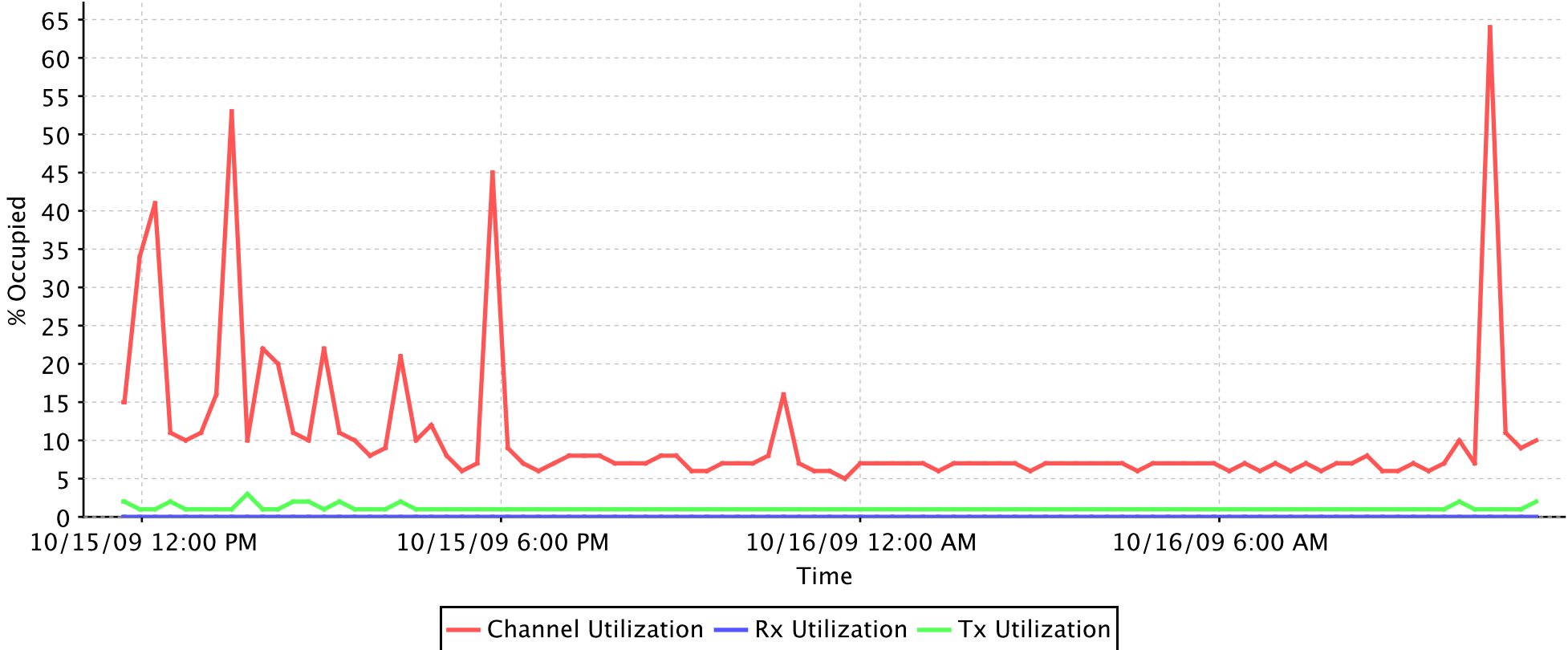
Radio Utilization of ics-ap-C114, 00:15:f9:5a:dc:40, 802.11b/g
